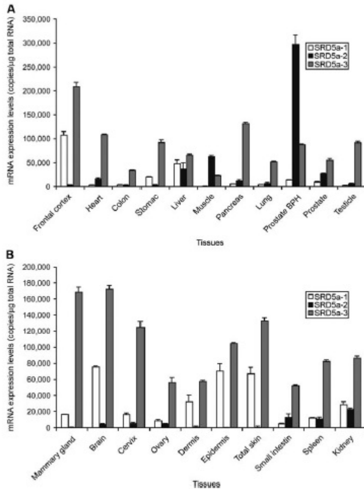
Figure 3 Comparison of mRNA expression levels of SRD5a-1, 2 and 3 in human tissues. Commercially available total RNA of male (A) and female (B) tissues was used to quantify mRNA expression levels of SRD5a-1, 2 and 3 by real-time PCR as described in the Materials and methods section. Data are expressed as mean \pm SEM of triplicate measurements.
