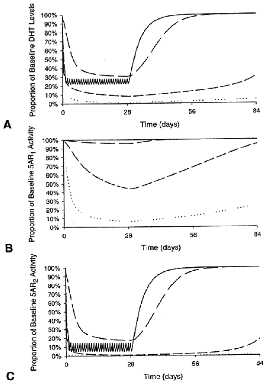
Figure 6. Predicted mean levels of dihydrotestosterone (DHT) (A), 5 \alpha -reductase type 1 (B), and 5 \alpha -reductase type 2 (C) suppression after daily doses of 5 mg finasteride ( solid line ) and 0.1 mg ( long-dashed line ), 1 mg ( short-dashed line ), and 10 mg ( dotted line ) GI198745 for 28 days.
