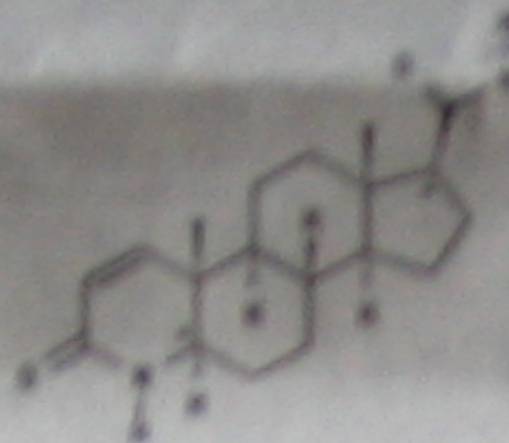
Chemical structure of Dutasteride
